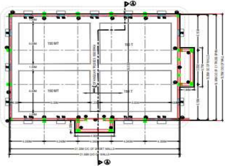
PLAN FOR 600 MT W.H. BLDG.
